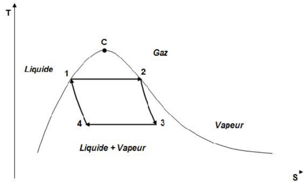
Figure 3. Cycle de Carnot
