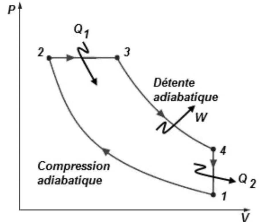
Figure 5.7. Cycle de Diesel
